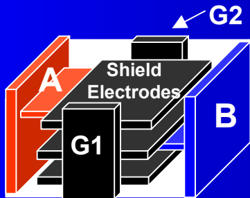
X2Y ® Capacitor
